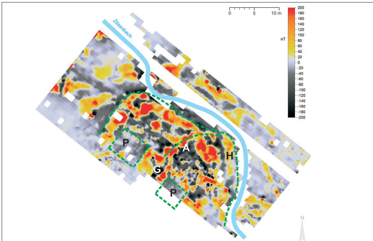
Figure 11: Magnetogram of the large slag concentration in the Zitzenbach Valley with meaningful anomalies. A: Headrace. G: Water wheel location. H: Slag heap. P: Location of a stamp mill or furnace. Survey: T. Riese (Posselt & Zickgraf Prospektionen GbR Marburg); cartography: M. Zeiler.
