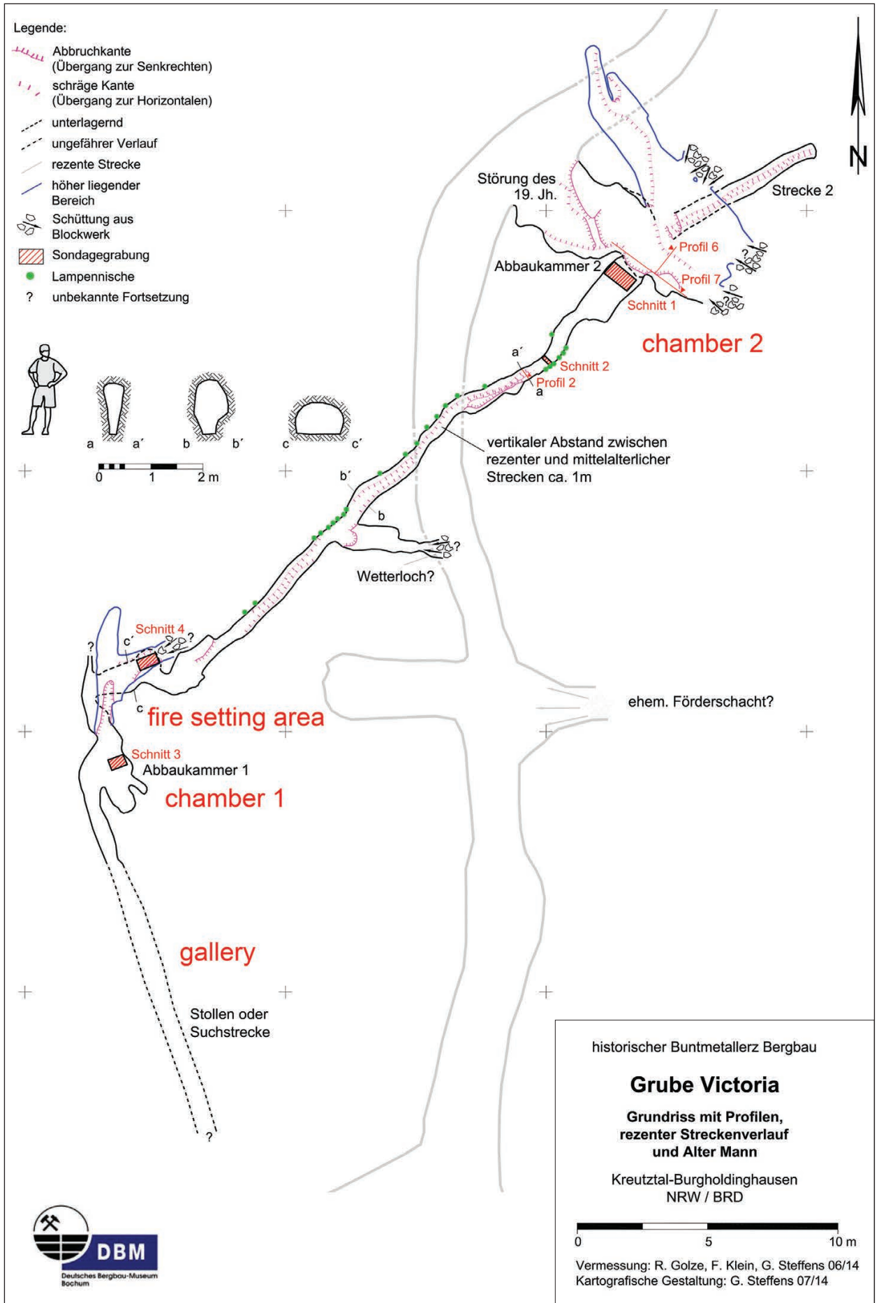
Figure 4: Ground plan of the medieval Alter Mann Victoria mine.
